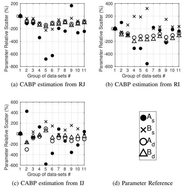
Fig. 4. Scattering of parameters of the used in CABP-HM: evolution along the eleven groups of data-sets acquired during three days of intermittent assessment. Parameter variability is written as a relative scatter (error) from the parameters resolved from the first group of data-sets
