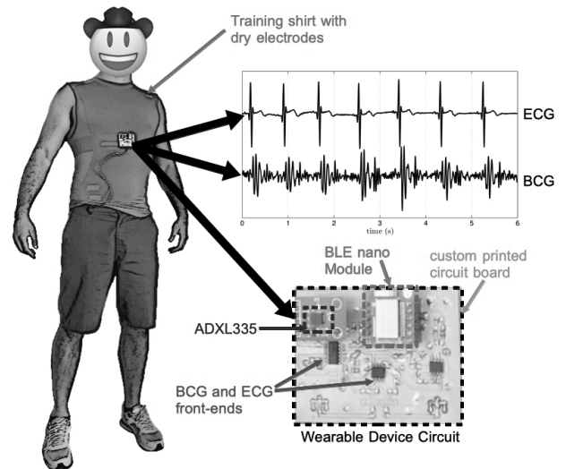
Fig. 1. Details of wearable device prototype [11] in a volunteer.
